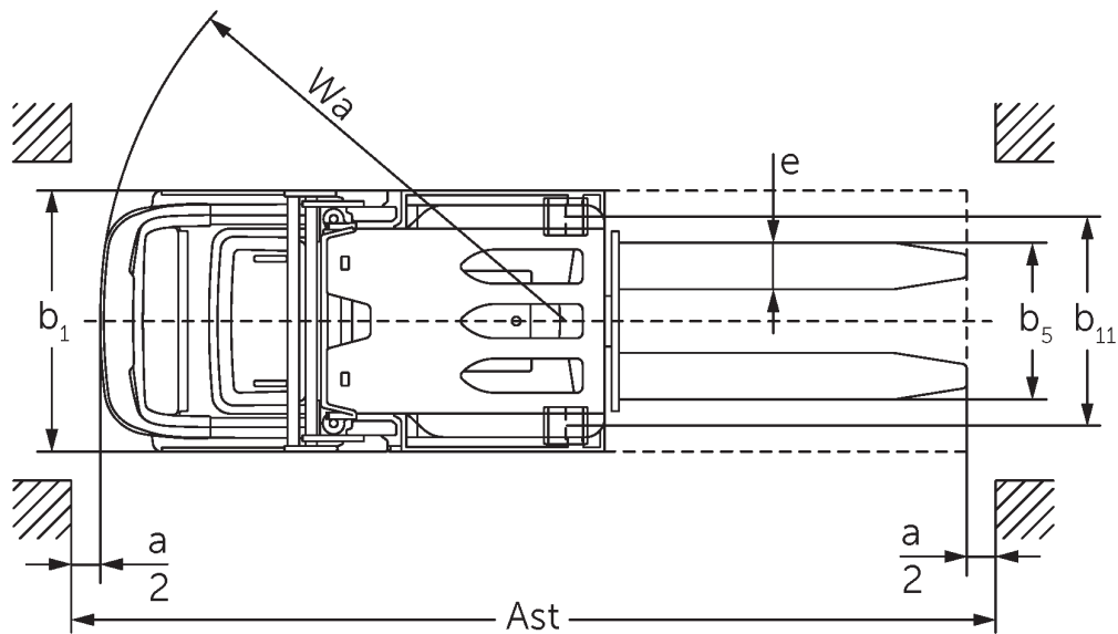
Figure shows EKS 110 Z 280 ZZ
