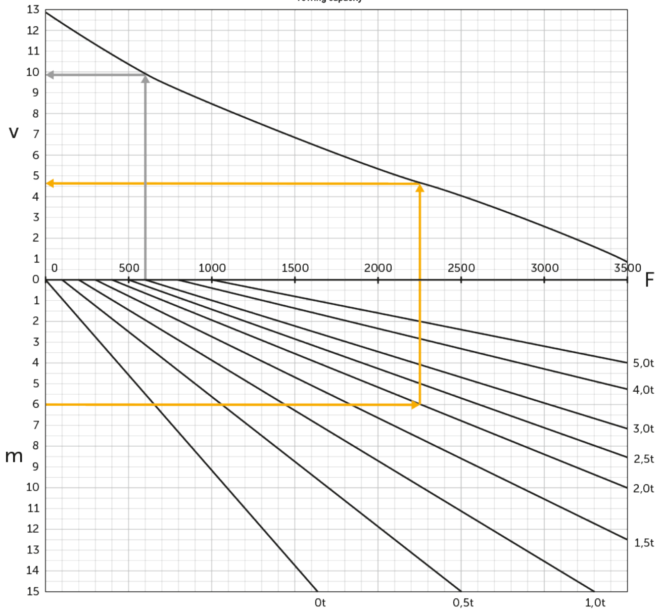
Towing capacity
