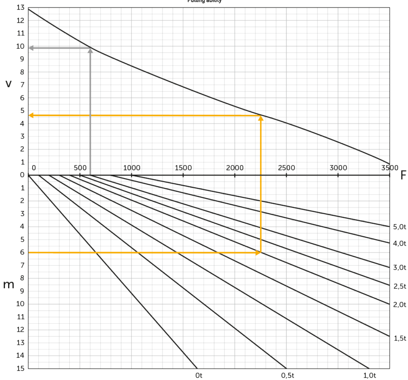
Pulling ability
