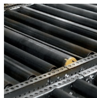
With pallet live storage, brake rollers control the speed of pallet transportation.
